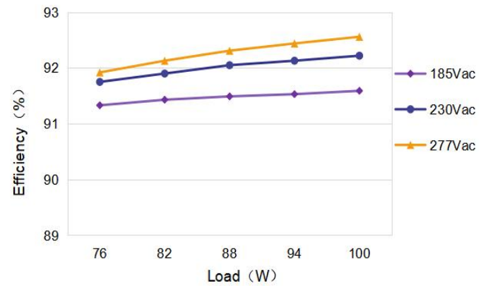
Typical Efficiency vs Load
