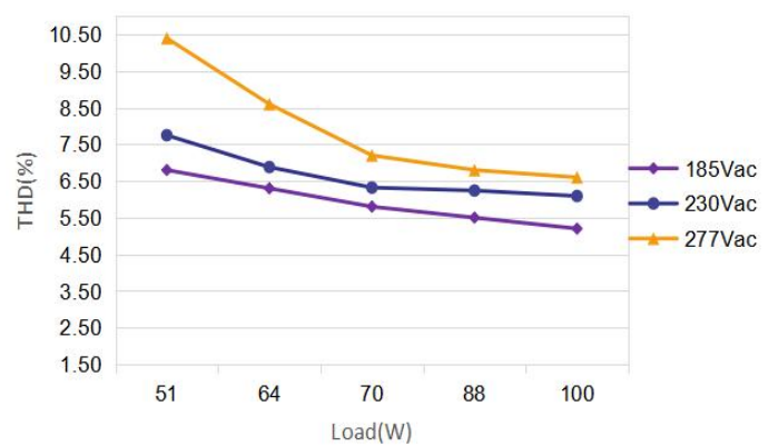
Typical THD vs Load
